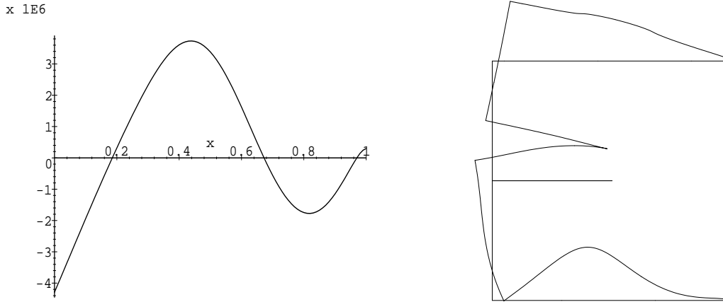
Figure 12: Resolution of (P_h) without constraint on \mathbf{h} - Optimal density h_2^{opt} ( Left ) and corresponding deformation ( Right ) - g_\psi(\mathbf{u}, \mathbf{h}^{opt}, \mathcal{X}_{\Gamma_h}) \approx 0.0383N/m .
