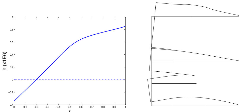
Figure 16: Resolution of (P_h) - Optimal density h_2^{opt} (Left) and corresponding deformation (Right) - g_\psi(\mathbf{u}, \mathbf{h}^{opt}, \mathcal{X}_{\Gamma_h}) \approx 0.0556N/m .
