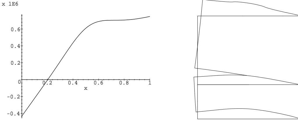
Figure 10: Resolution of (P_h) - Optimal density h_2^{opt} (Left) and corresponding deformation (Right)- g_\psi(\mathbf{u}, \mathbf{h}^{opt}, \mathcal{X}_{\Gamma_h}) \approx 0.0353N/m .
