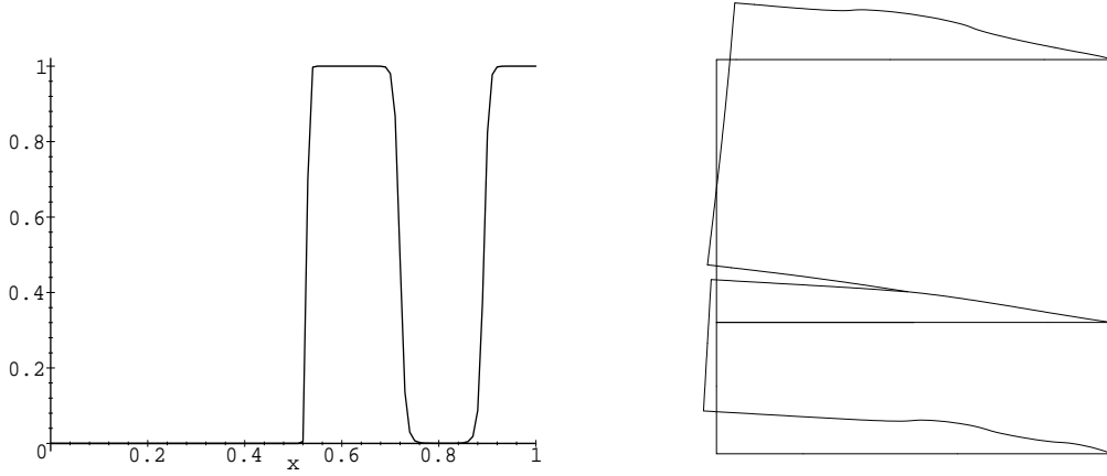
Figure 7: Resolution of (RP_{\Gamma_h}) - Optimal density s^{opt} (Left) and corresponding deformation (Right)- g_\psi(\mathbf{u}, \mathbf{h}, s^{opt}) \approx 0.1050 N/m .
