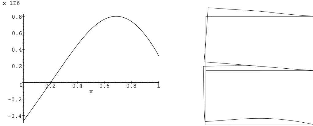
Figure 11: Resolution of (P_h) - Optimal density h_2^{opt} ( Left ) and corresponding deformation ( Right ) - g_\psi(\mathbf{u}, \mathbf{h}^{opt}, \mathcal{X}_{\Gamma_h}) \approx 0.00679N/m .
