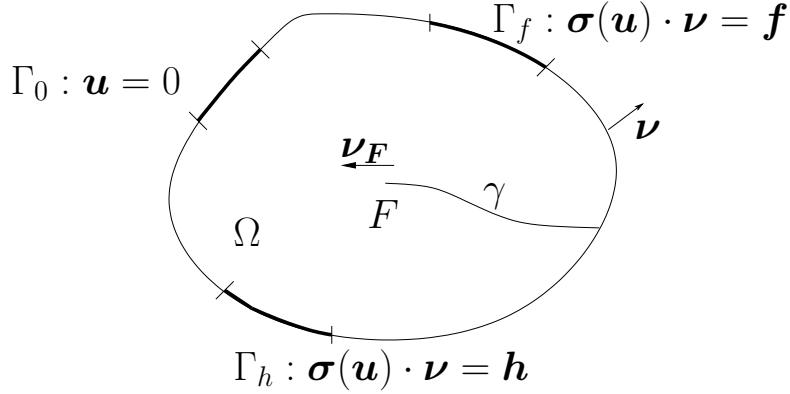
Figure 1: Illustration of the problem (P_{\Gamma_h}) : Optimization of the location of \Gamma_h , the support of the extra load \mathbf{h} in order to minimize the energy release rate.
