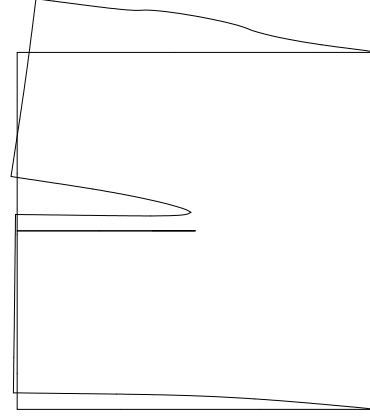
Figure 3: Initial and deformed configurations of S without additional extra force (i.e., \mathcal{X}_{\Gamma_h} = 0 ) and a = 0.5 : g_\psi(\mathbf{u}, \mathbf{h}, 0) \approx 1.147N/m .
