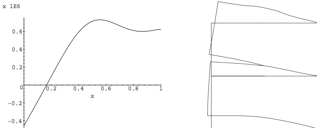
Figure 9: Resolution of (P_h) - Optimal density h_2^{opt} ( Left ) and corresponding deformation ( Right )- g_{\psi}(\mathbf{u}, \mathbf{h}^{opt}, \mathcal{X}_{\Gamma_h}) \approx 0.4328N/m .
