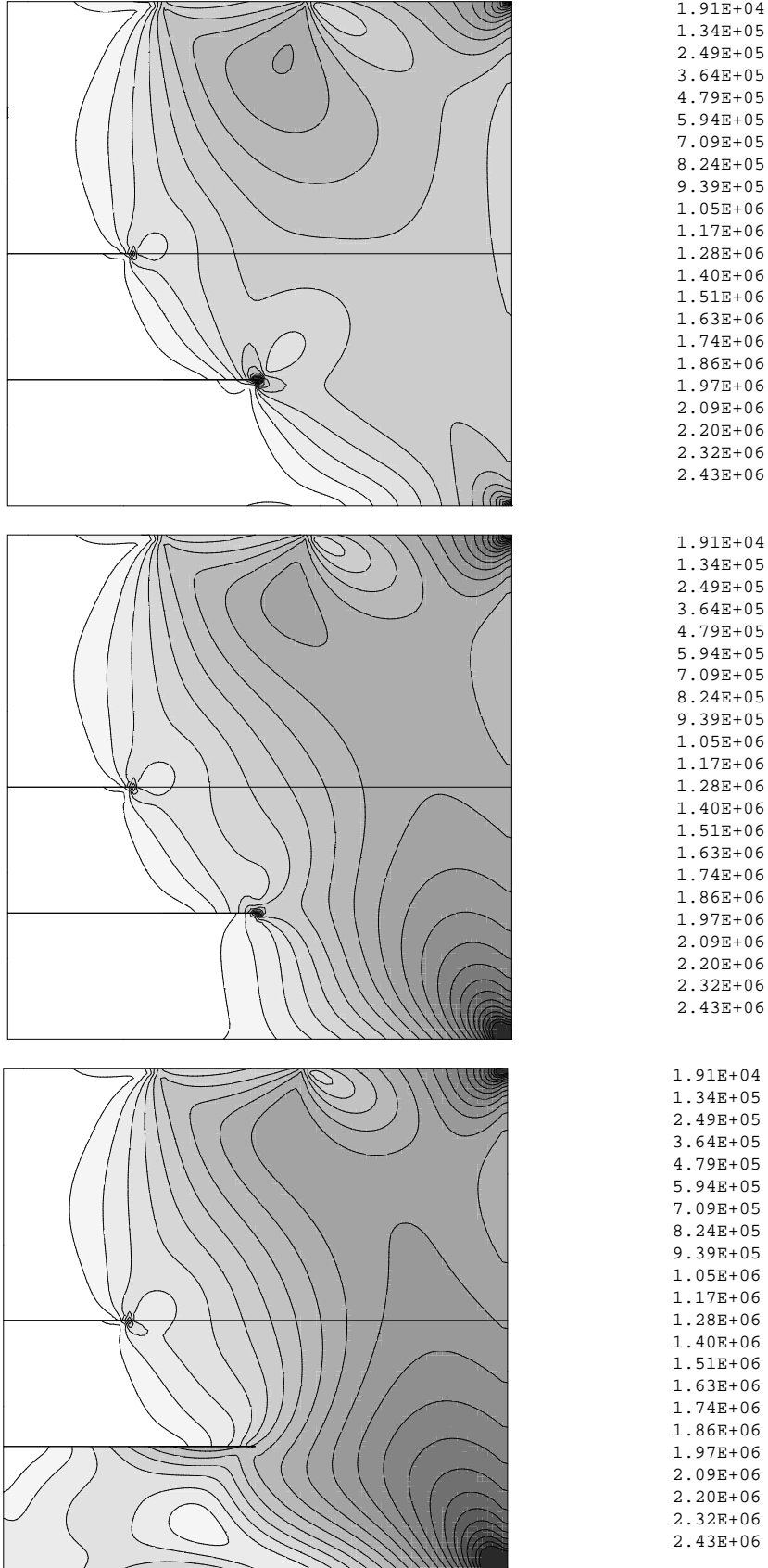
Figure 15: Iso-values of the Von Mises Stresses on \Omega - a ) without extra-force g_\psi(\mathbf{u}, \mathbf{h}, 0) \approx 0.232N/m ( Top ) - b ) from (RP_{\Gamma_h}) g_\psi(\mathbf{u}, \mathbf{h}, s^{opt}) \approx 0.102N/m ( Mid ) and c ) from (P_h) g_\psi(\mathbf{u}, \mathbf{h}^{opt}, \mathcal{X}_{\Gamma_h}) \approx 0.0556N/m ( Bottom ).
