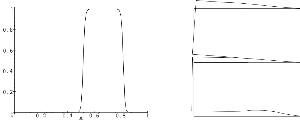
Figure 8: Resolution of (RP_{\Gamma_h}) - Optimal density s^{opt} ( Left ) and corresponding deformation ( Right )- g_{\psi}(\mathbf{u}, \mathbf{h}, s^{opt}) \approx 0.0281N/m .
