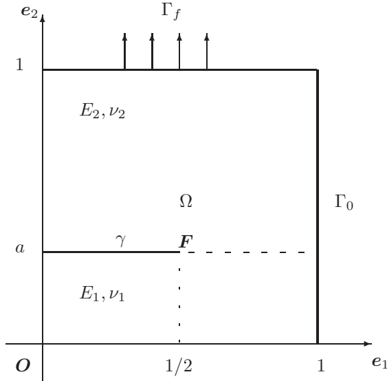
Figure 2: Setting of the problem.
