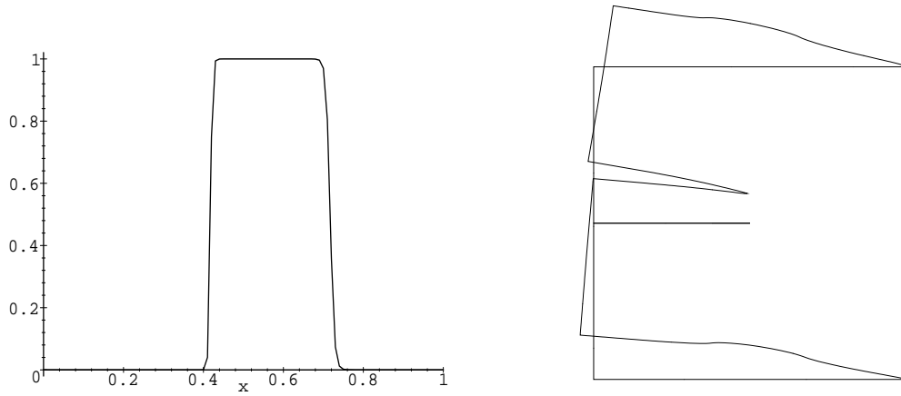
Figure 4: Resolution of (RP_{\Gamma_h}) - Optimal density s^{opt} ( Left ) and corresponding deformation ( Right ) - g_\psi(\mathbf{u}, \mathbf{h}, s^{opt}) \approx 0.4641N/m .
