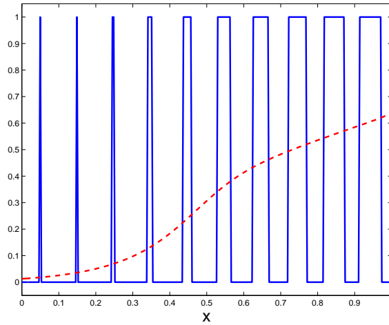
Figure 14: Penalization of the limit density s^{lim} in the case (a_1, a_2) = (1/2, 1/2) by a characteristic function \mathcal{X}_{\Gamma_h}^{(10)} .
