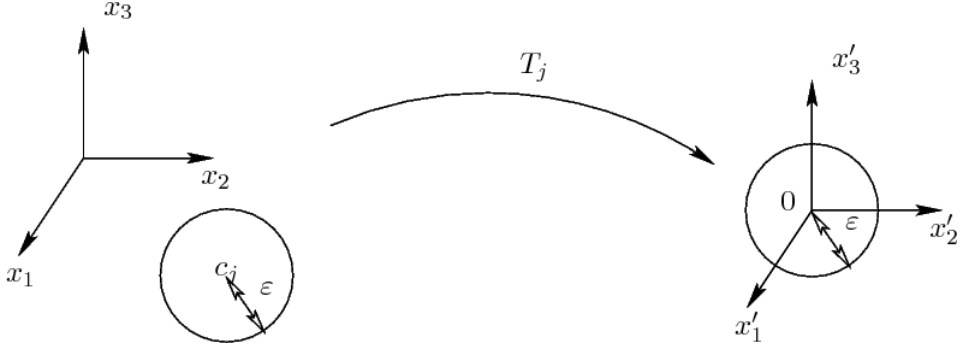
FIGURE 2. Notation for the translation of the coordinates system.
