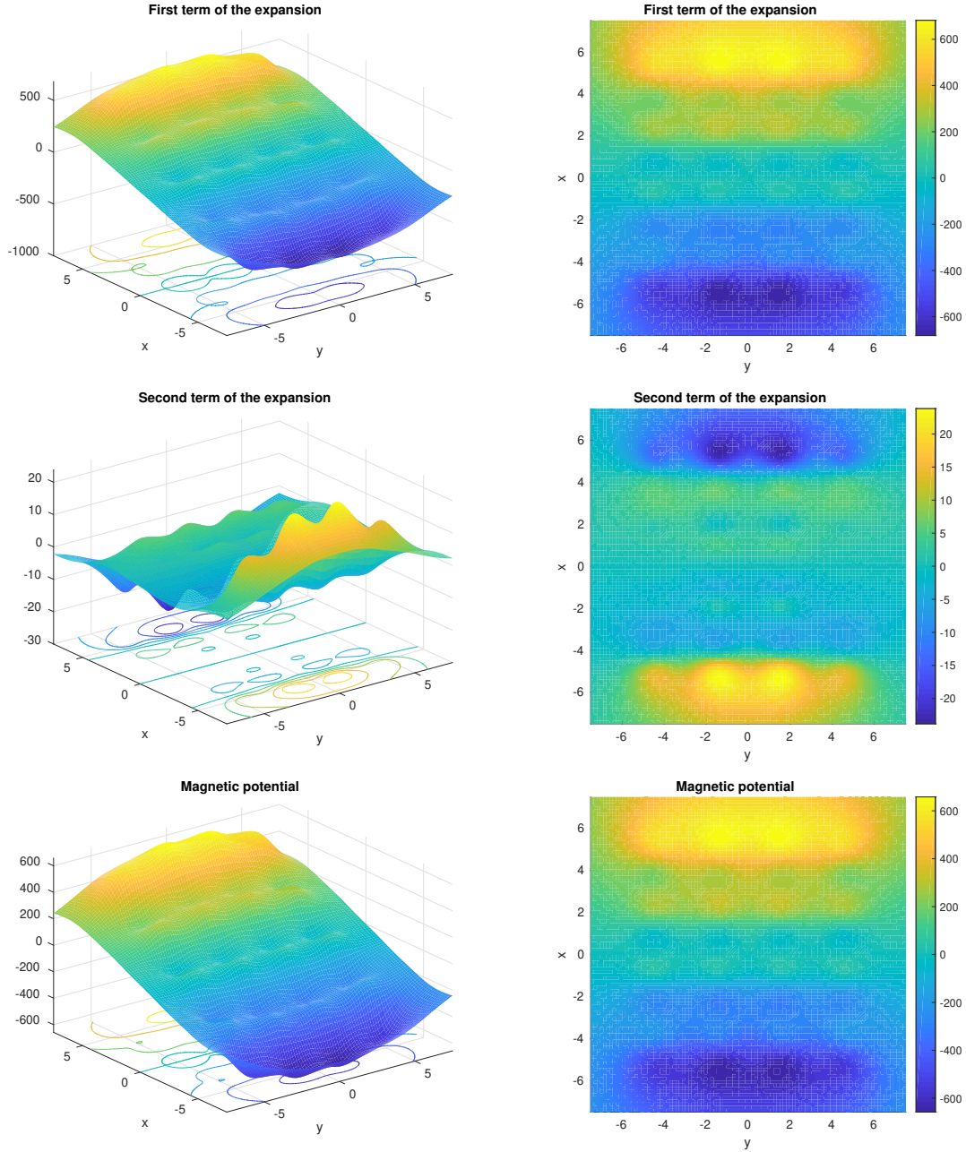
FIGURE 9. Cube of 64 equidistant particles. From top to bottom : first term in the series expansion of the magnetic potential, second term in the series expansion and approximation of the magnetic potential obtained by summing the first two terms of the series expansion. From left to right : three-dimensional shaded surface representation and two-dimensional representation of the three quantities.
