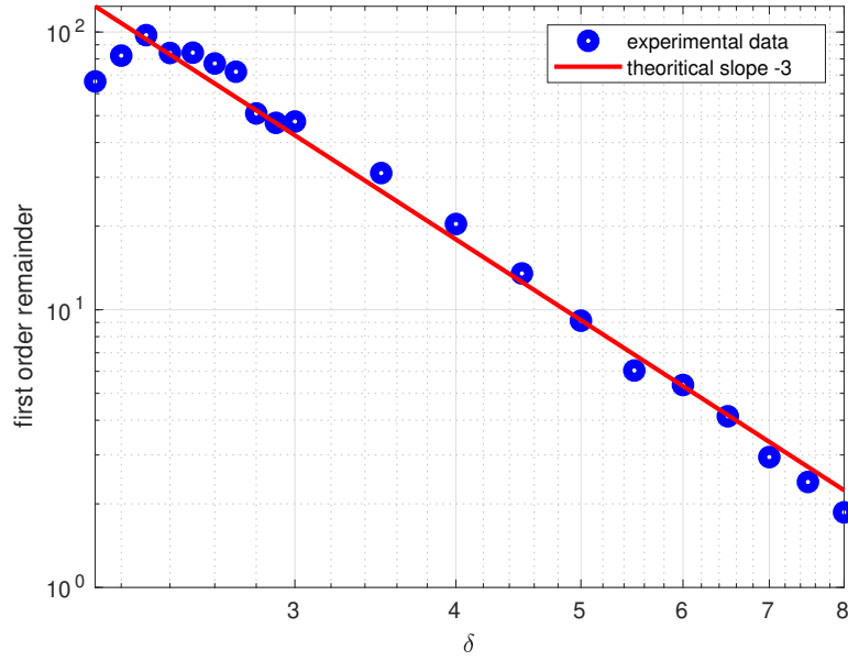
FIGURE 6. Values of \mathfrak{E} as a function of the distance \delta between the two spherical particles in a log-scale. The slope of the solid line is -3 .
