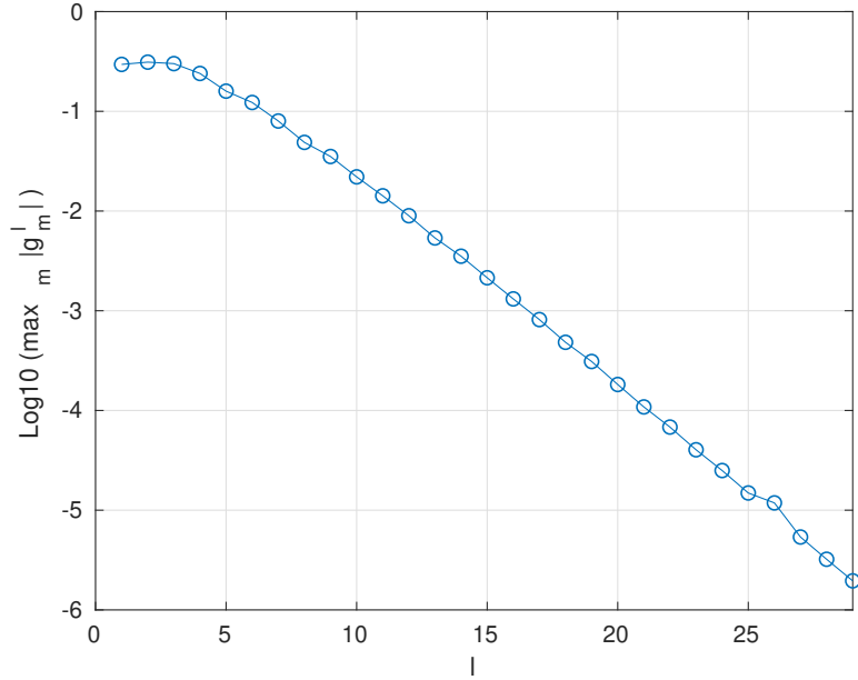
FIGURE 5. Values of the decimal logarithm of \max_{m=-\ell, \dots, \ell} |g_\ell^m| for \ell = 1, \dots, 29 for \mu_p = 10 , \varepsilon = 1 and u = c_k - c_j = (1, 1, 1)^\top .
