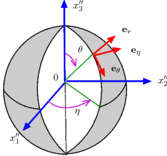
FIGURE 10. Notation for the spherical coordinates.
