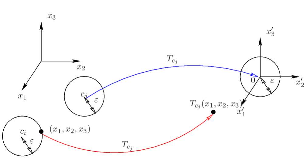
FIGURE 3. Effect of the translation of the coordinates system for several particles.
