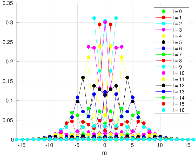
FIGURE 4. Values of |g_\ell^m| for m = -\ell, \dots, \ell and \ell = 0, \dots, 16 for \mu_p = 10 , \varepsilon = 1 and u = c_k - c_j = (1, 1, 1)^\top .
