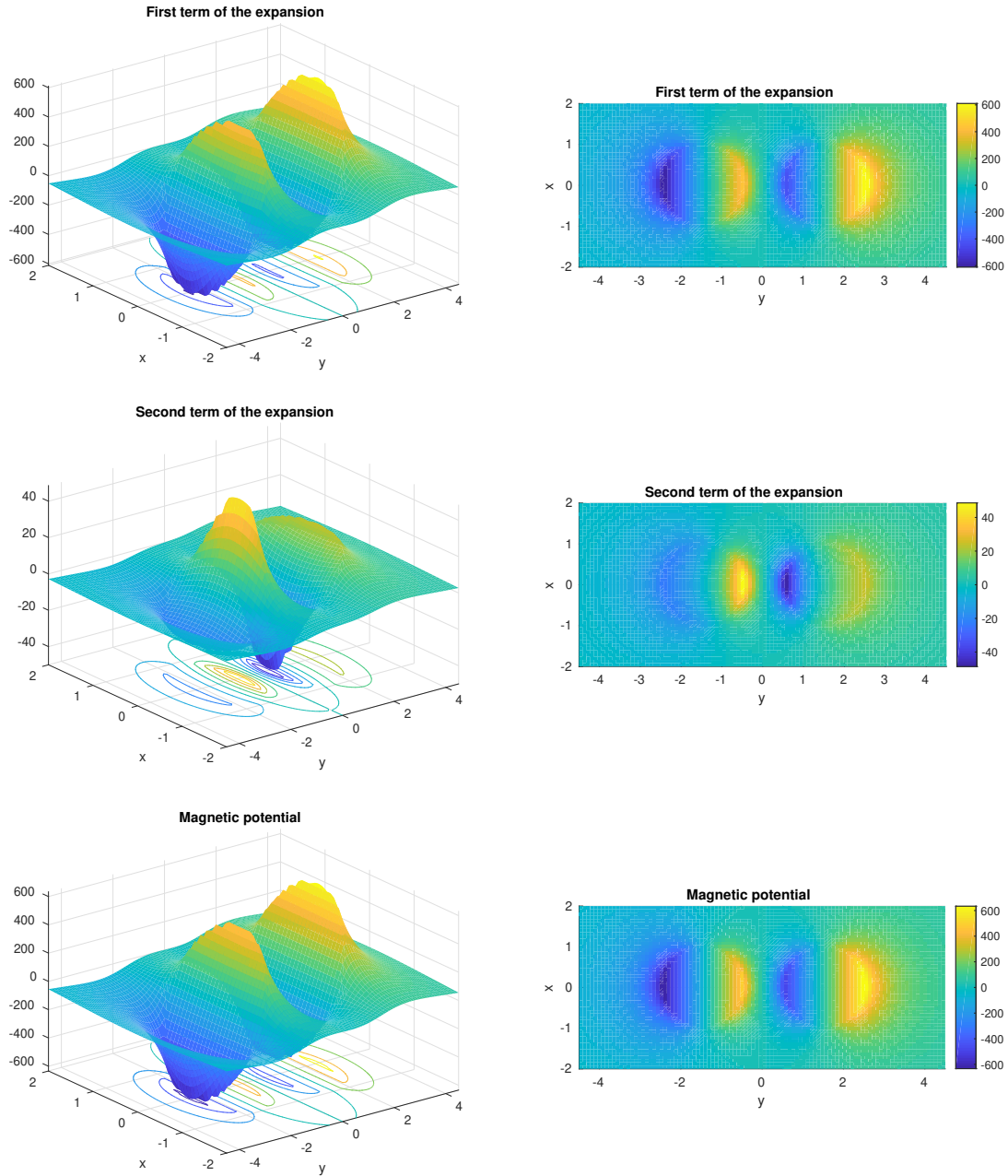
FIGURE 8. Two particles. From top to bottom : first term in the series expansion of the magnetic potential, second term in the series expansion and approximation of the magnetic potential obtained by summing the first two terms of the series expansion. From left to right : three-dimensional shaded surface representation and two-dimensional representation of the three quantities.
